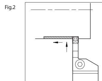
Fig.2 Traversing subsequent to grooving. (Grooving depth under 0.5mm : At Finishing)
